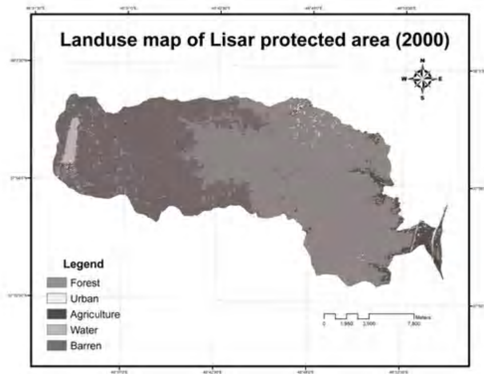
Fig. 3. land use map of Lisar protected area (2000)
