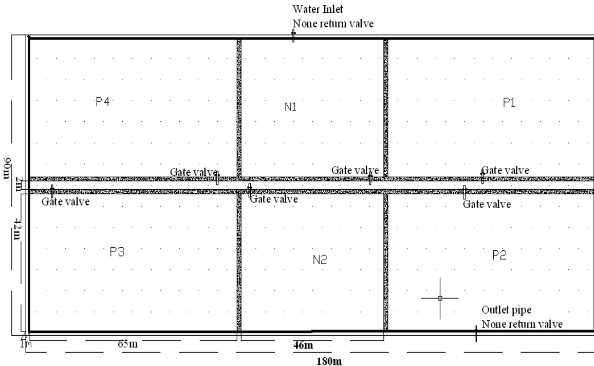
Fig. 3. Layout of fish ponds
