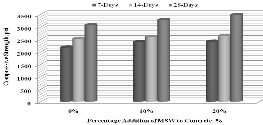
Fig. 2. Compressive strength of concrete with addition of MSW
