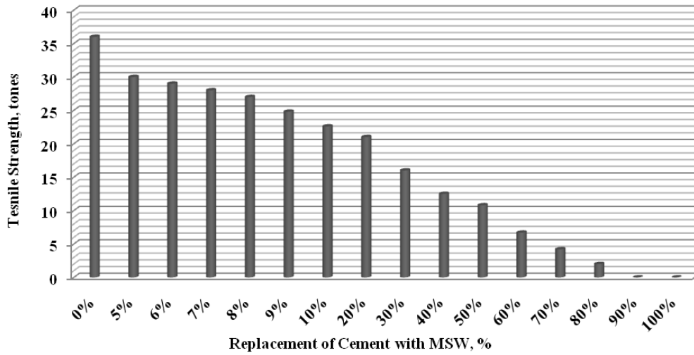
Fig. 4. Tensile Strength of concrete with partial replacement of cement with MSW
