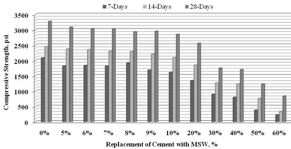
Fig. 1. Compressive strength of concrete with partial replacement of cement with MSW
