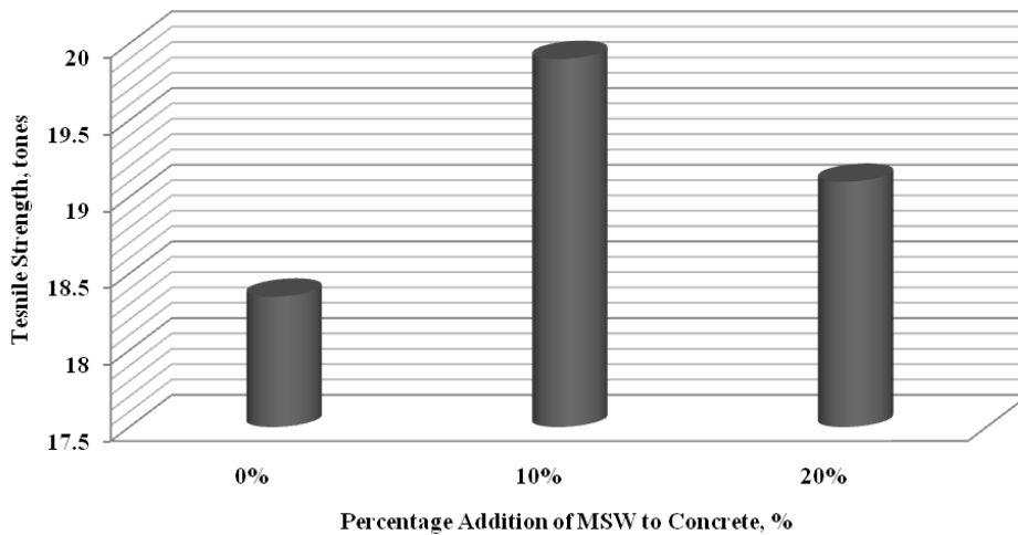
Fig. 5. Tensile Strength of concrete with addition of MSW
