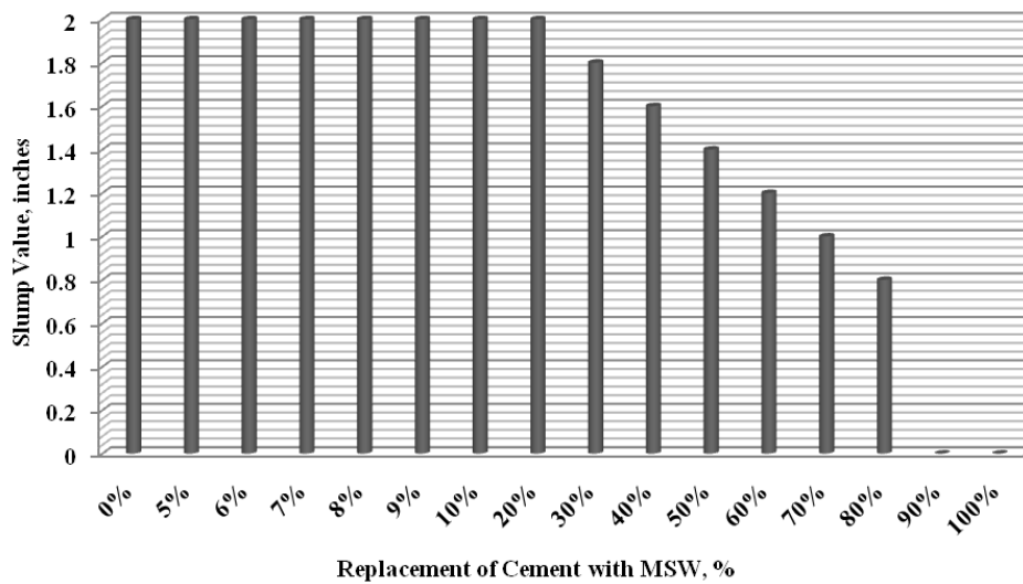
Fig. 3. Results of slump test of concrete with partial replacement of cement with MSW
