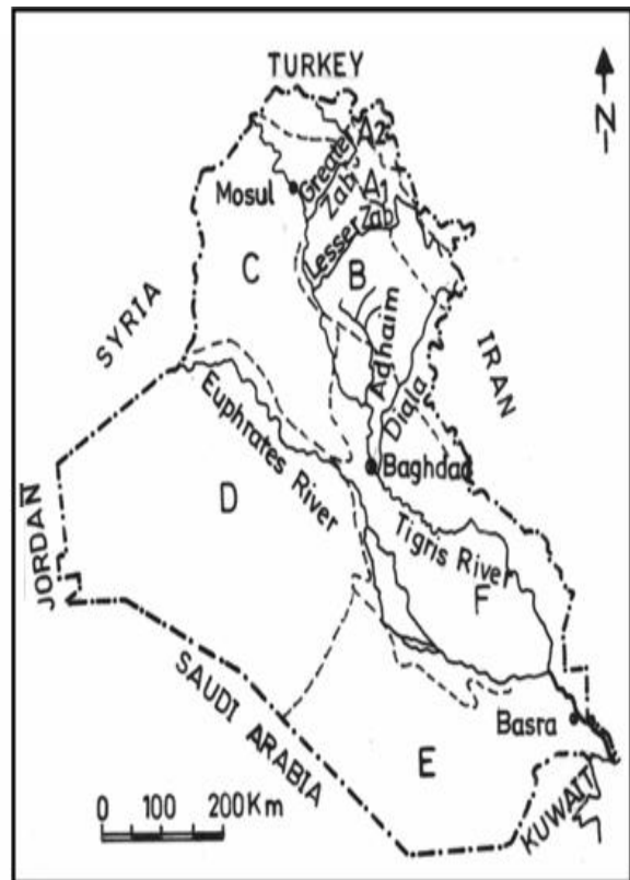
Fig. 1. The physiographic provinces of Iraq. Provinces are: Zagros mountains (A1, folded zone; A2, nappe zone), Foothills (B), Jezira (C), Northern (D) and Southern (E) deserts, and the Mesopotamian Plain (F) after Berry et al. (1970)
