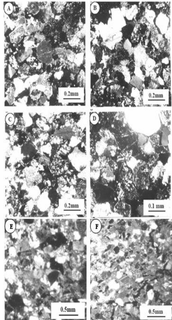
Fig. 3. Photomicrographs of selected sandstone samples of Injana Formation; (A) General view showing the common presence of carbonate lithic fragments generally rounded to sub-rounded, chert rock fragments and few poly-and monocrystalline quartz grains; (B) Both fresh and altered feldspar grains with rounded quartz; (C) Fresh feldspar, mono and polycrystalline quartz grains, chert, argillaceous and carbonate lithic fragments; (D) Chert of microcrystalline (ch) and radiolarian types (R); (E)&(F) Photomicrographs of selected sandstone samples of the Fatha Formation showing quartz, both mono and polycrystalline with chert rock fragments and little feldspar in carbonate (calcite) cement, some of calcite cement is re-crystallized
